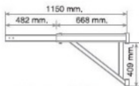
HORIZONTAL SUPPORT
